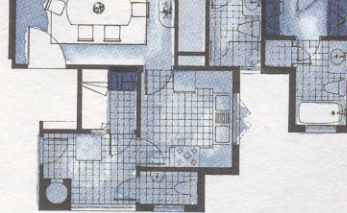
Type B5 119m 2 (incl. terrace 8m 2 )
