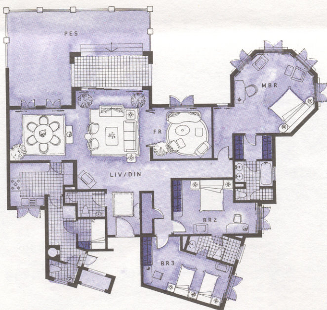
Type C4 212m 2 (incl. terrace 11m 2 ) 252m 2 (incl. PES 40m 2 )
